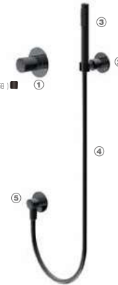
7025B-2 (W0125B-2+R0025B+S025B+R22+B2125B) ■ Concealed-shower mixer (1-function) ① W0125B-2 : Concealed mixer Ceramic cartridge: 35mm ② R0025B : Shower holder ③ S025B : Hand shower, Brass, 1-function ④ R22 : Hose, 150cm, PVC ⑤ B2125B : Shower outlet
