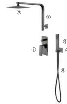
7721BN-2 (W0221BN-2 + B1295BN + P73BN + B2214BN + S017BN + R28BN) ■
